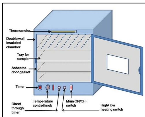
Figure 2.1 Hot Air Oven
